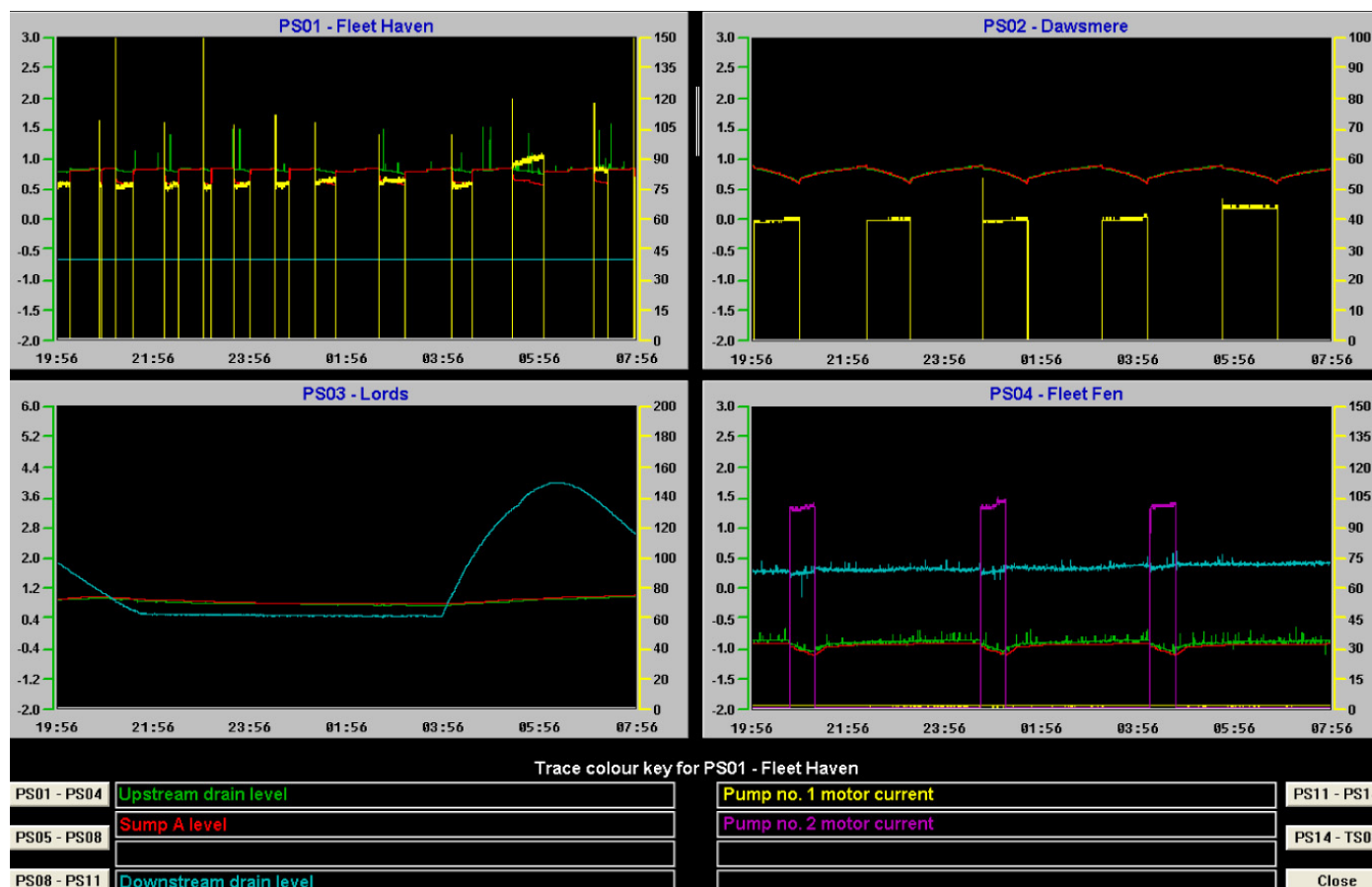
SCADA screens showing trends and events
