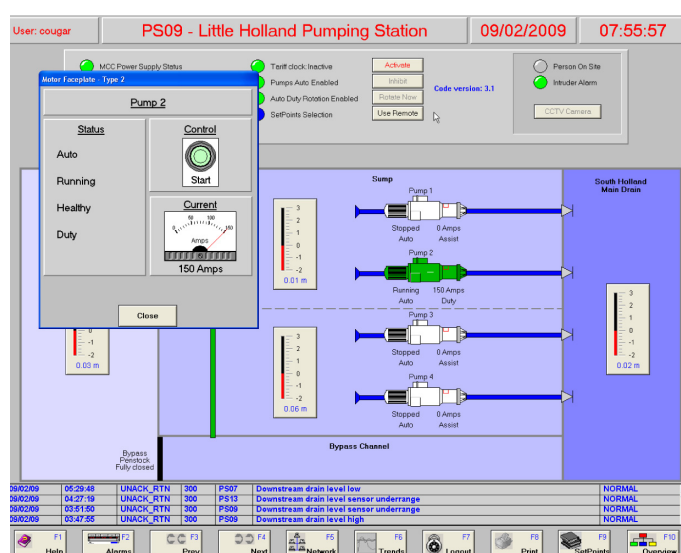
Equipment status displays
